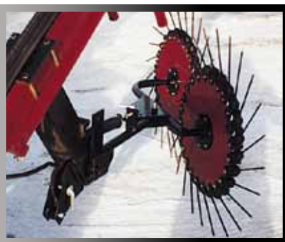
A 2 or 3 wheel center kicker assembly is optional for the Hi-Capacity rakes.
